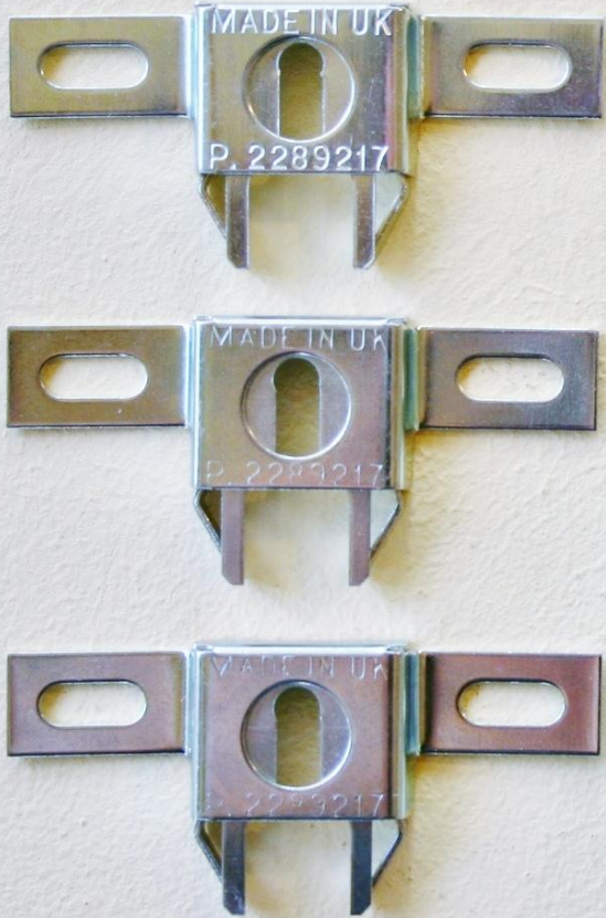
The SpringLOCK (2 Components) Bridge & Locking Spring Insert
